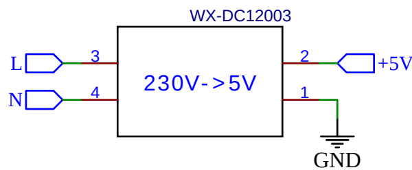
Power Supply 230v
