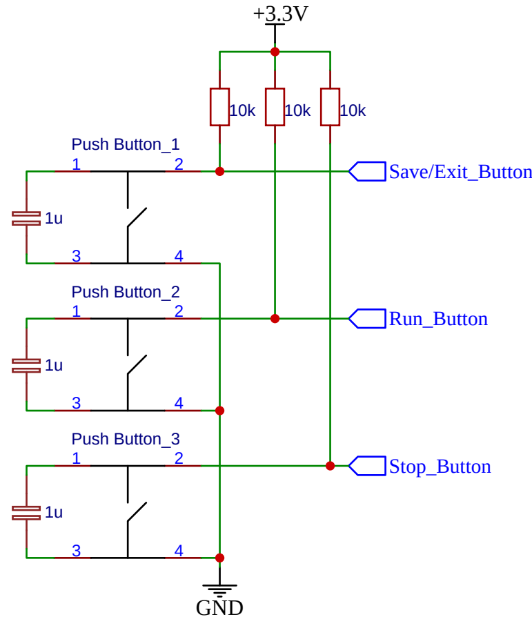
Push Buttons
