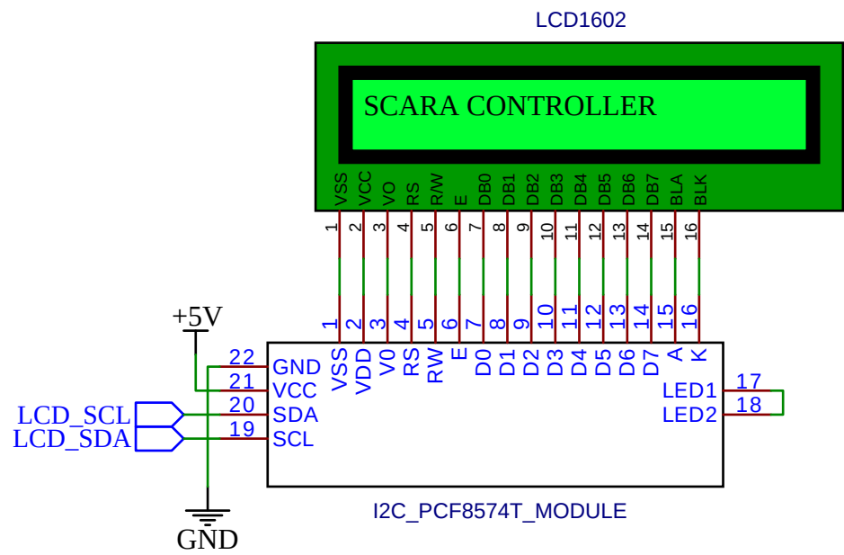
LCD Character With I2C Interface
