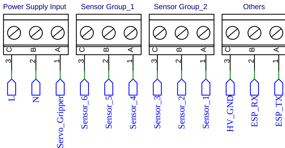
Bottom Screw Terminals
