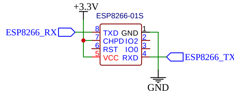
ESP8266-01S
