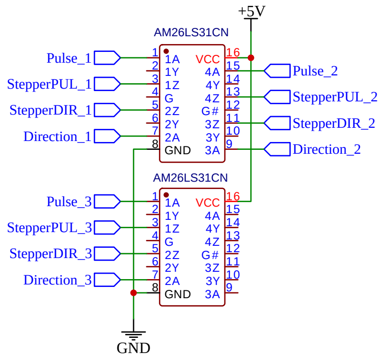
Output Pulse/Direction LineDrive
