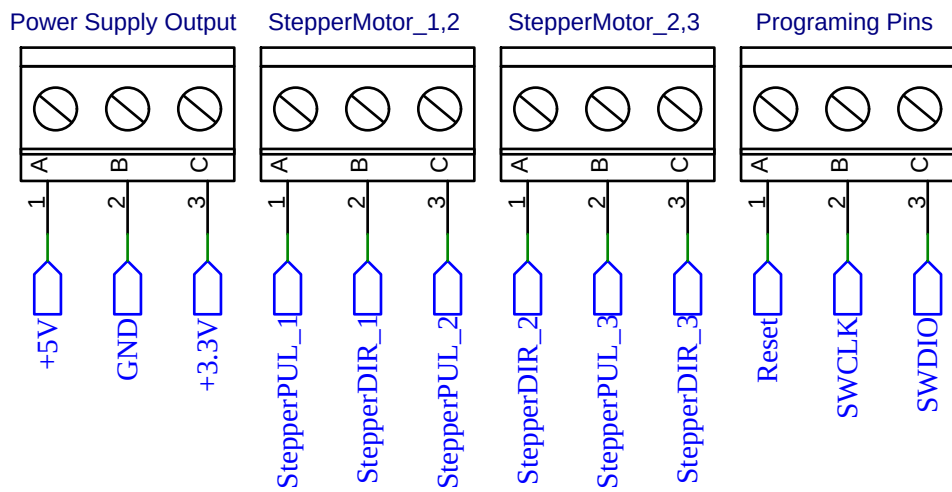
Top Screw Terminals
