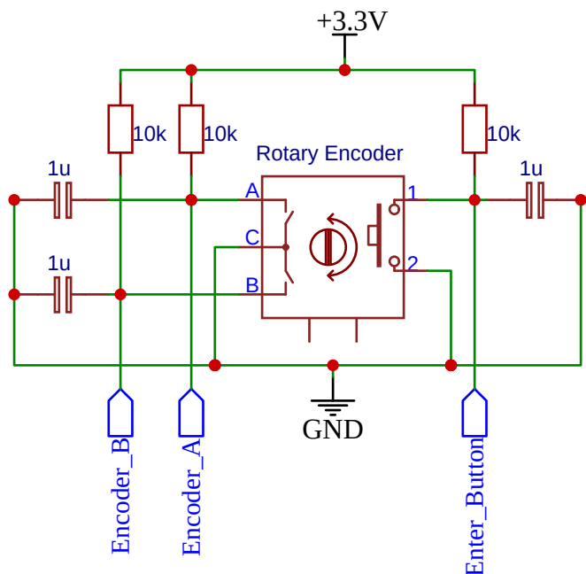
Rotary Encoder
