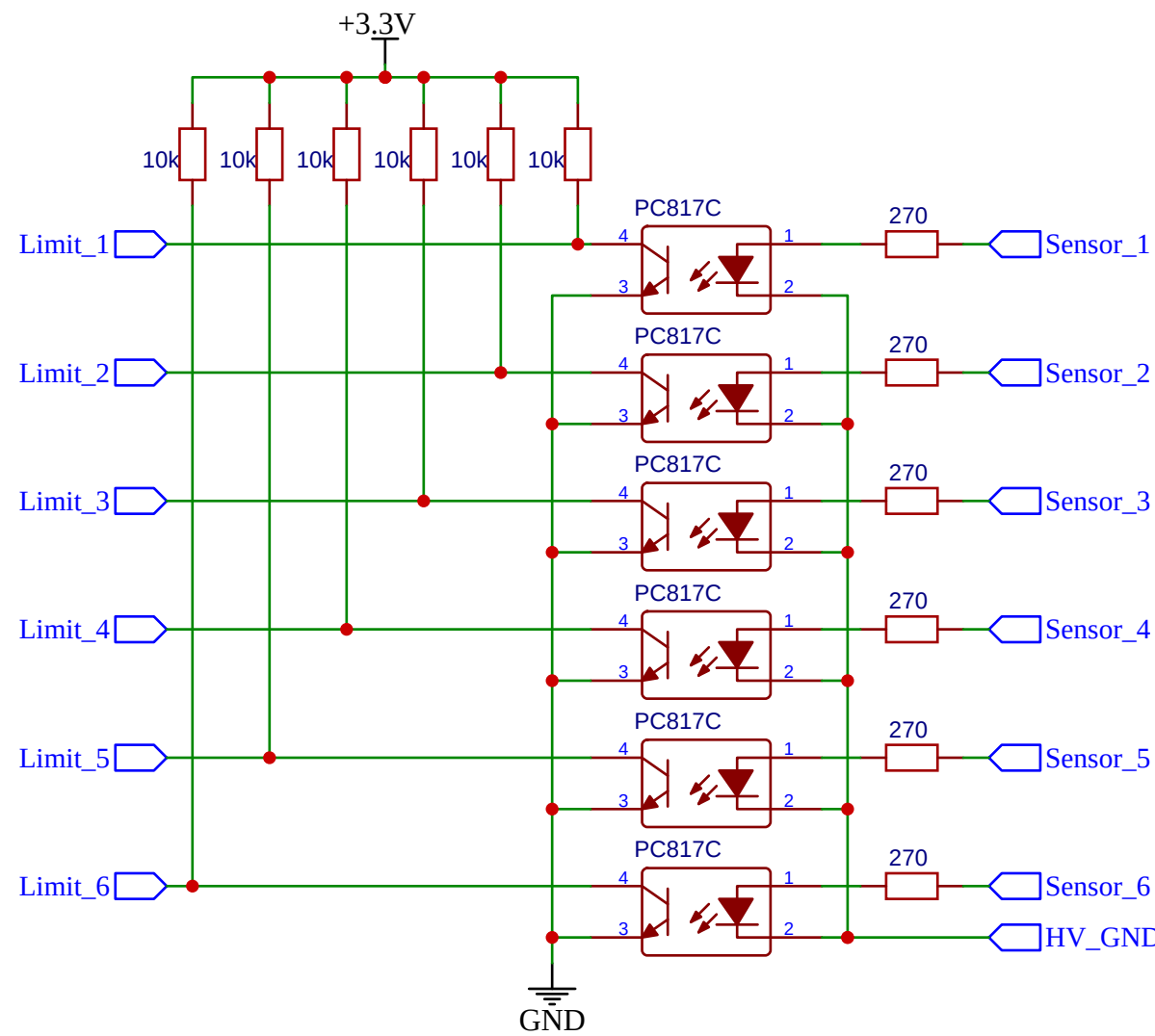
Input Homing Sensors
